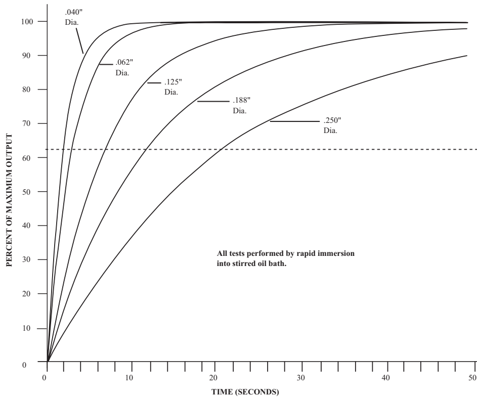
Response Times of Sheathed, Grounded Thermocouples
